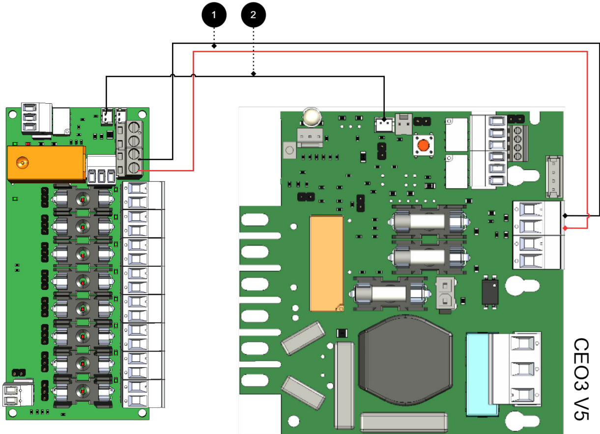
Figure 2. Connect the card as shown in the picture.
