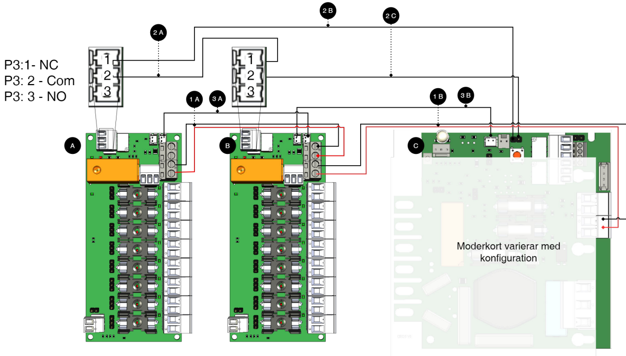
Figure 10. Connecting additional option cards to the motherboard
