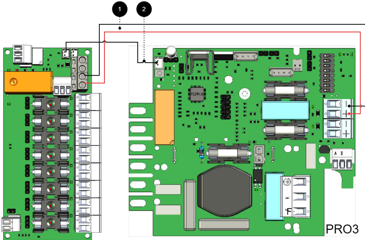
Figure 8. Connect the card as shown in the picture.
